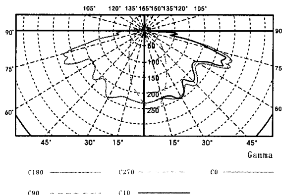
Intensity [cd/1000lm] Polar diagram NBDD-01B 400W
